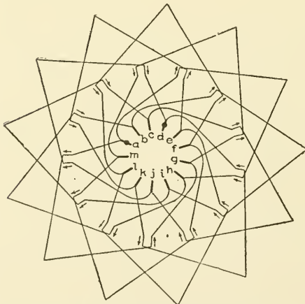
Fig. 139. Diagram Showing the Effect of Wrong Connections to Commutator Bars
